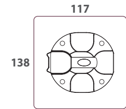
BASE PILAR
