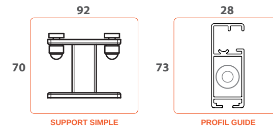
SUPPORT SIMPLE
