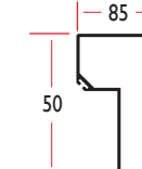
Profil Support Lame
